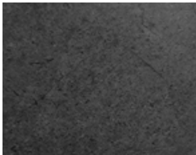
Ocean Basalt
